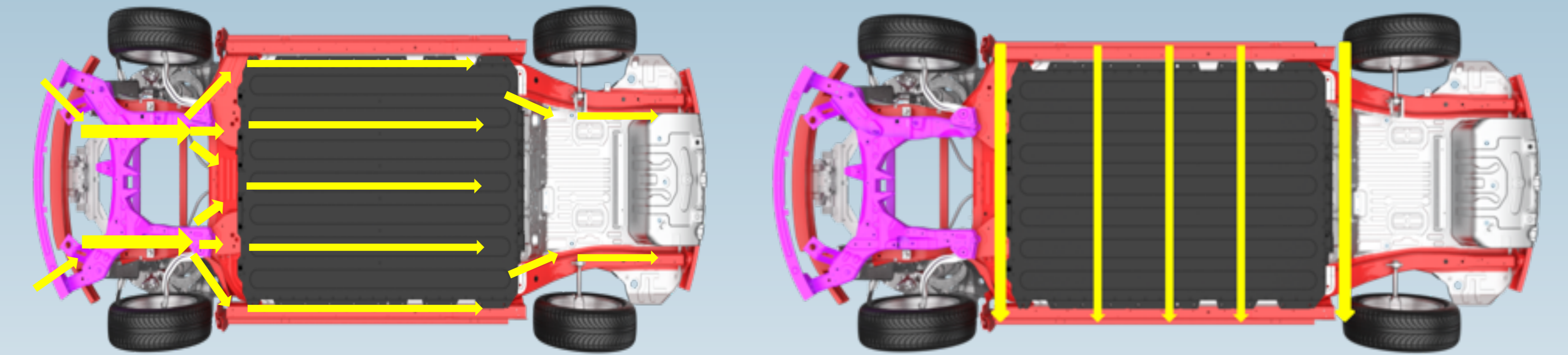
Force transmission path exclusively for pure EV ensures better protection
